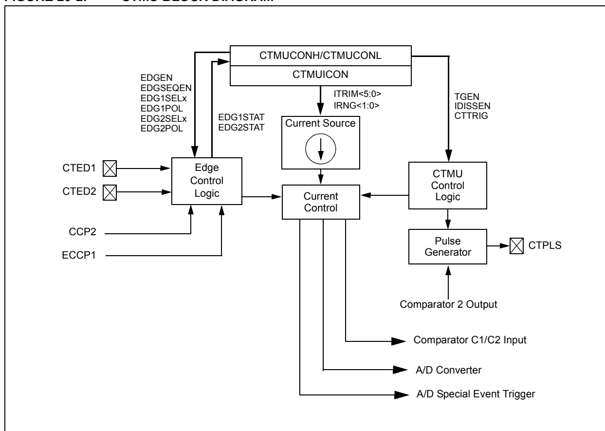
FIGURE 20-1: CTMU BLOCK DIAGRAM
