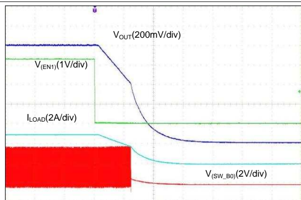
R_{LOAD} = 0.33\text{ }\Omega Time (100 \mu\text{s}/\text{div} ) Slew-Rate = 3.8\text{ mV}/\mu\text{s}
