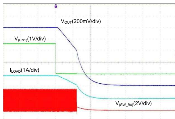
I_{OUT} = 0.5\text{ }\Omega Time (100 \mu\text{s}/\text{div} ) Slew-Rate = 3.8\text{ mV}/\mu\text{s}
