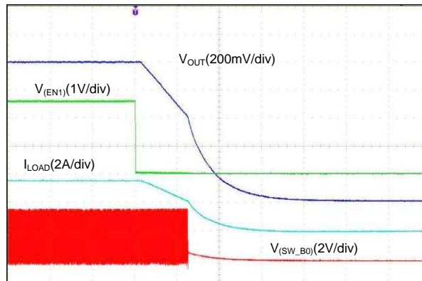
R_{LOAD} = 0.25\text{ }\Omega Time (100 \mu\text{s}/\text{div} ) Slew-Rate = 3.8\text{ mV}/\mu\text{s}
