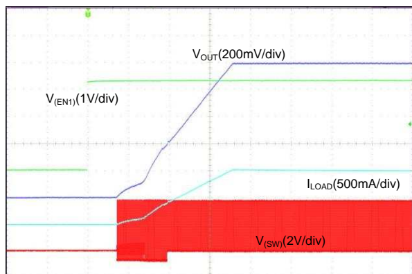
R_{LOAD} = 1\text{ }\Omega Time (100 \mu\text{s}/\text{div} ) Slew-Rate = 3.8\text{ mV}/\mu\text{s}
