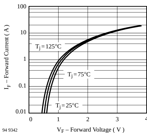
Figure 3. Max. Forward Current vs. Forward Voltage
