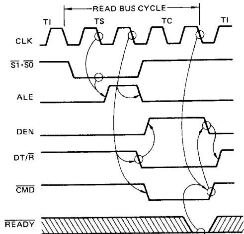
Fig. 6 — IDLE-READ-IDLE BUS CYCLES WITH MB = 0
