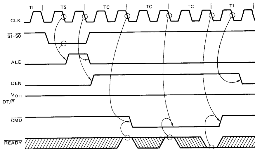
Fig. 10 – IDEL-WRITE-IDLE BUS CYCLES WITH MB = 1
