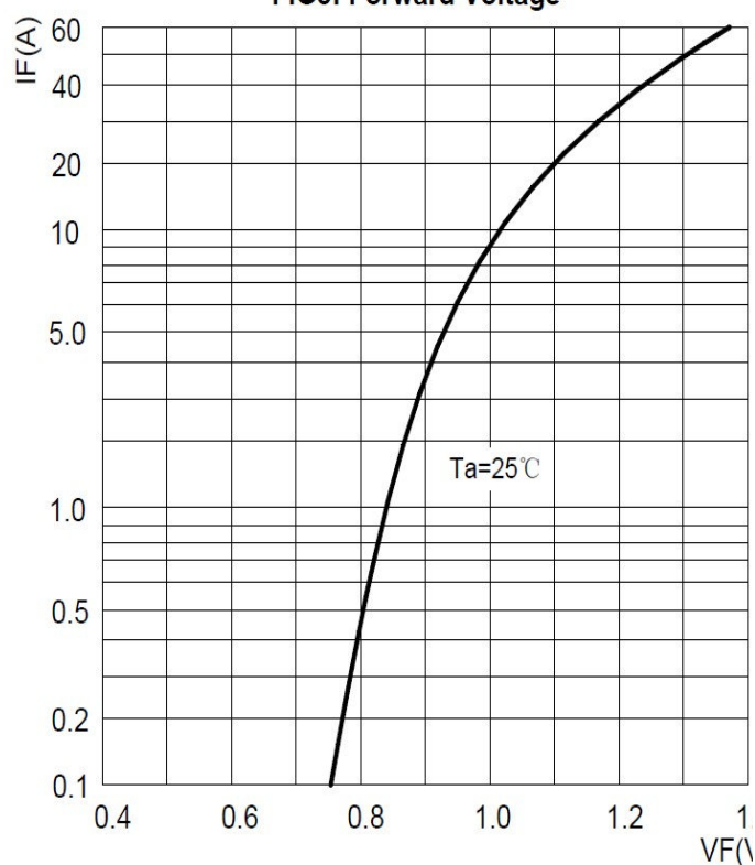
FIG3: Forward Voltage
