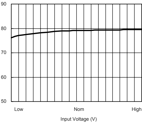
Efficiency vs Input Voltage ( Dual Output )
