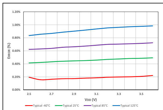
FIGURE 40-89: Typical FVR Voltage 1x Error, PIC16LF19155/56/75/76/85/86 Only.
