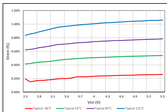
FIGURE 40-90: Typical FVR Voltage 1x Error, PIC16F19155/56/75/76/85/86 Only.
