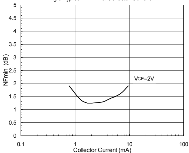
Fig.5 Typical NFmin &amp; Collector Current
