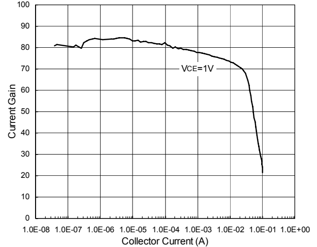
Fig.2 Typical Forward Current Gain &amp; Collector Current
