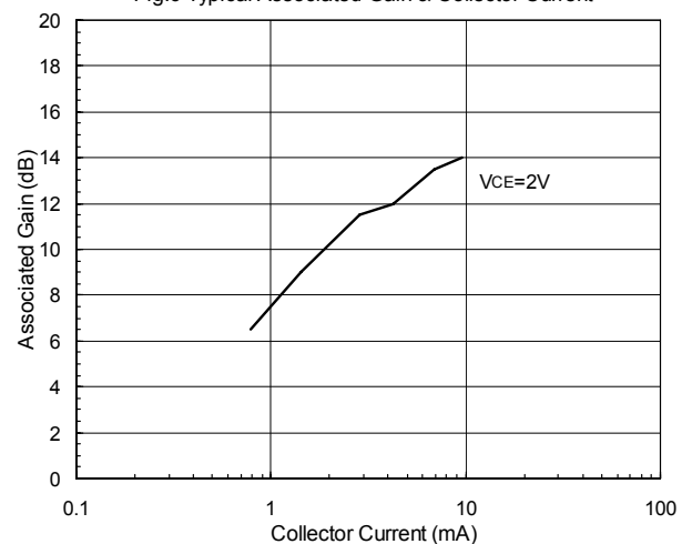
Fig.6 Typical Associated Gain &amp; Collector Current
