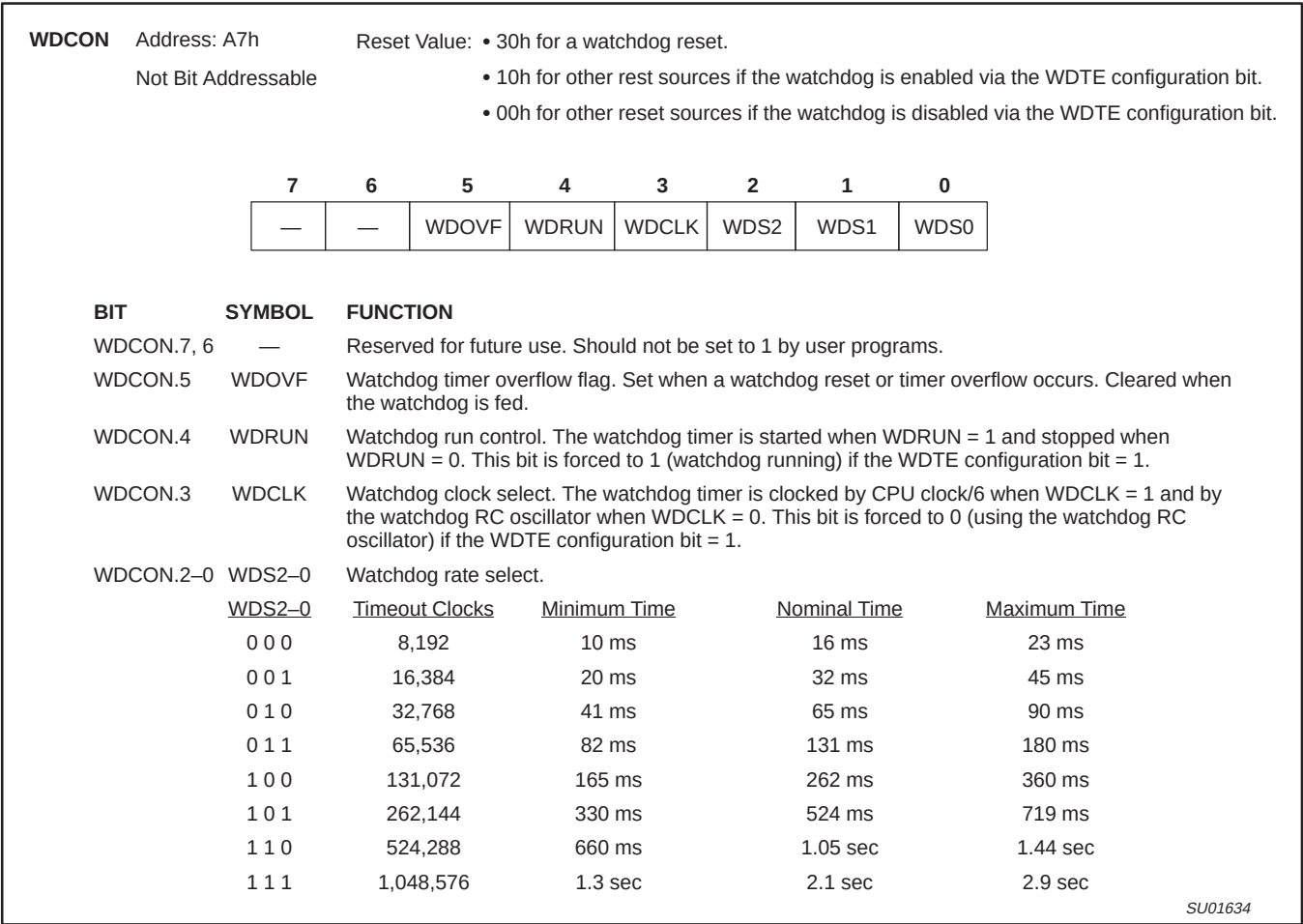
Figure 37. Watchdog Timer Control Register (WDCON)
