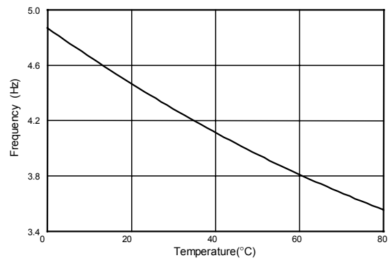
LED Flashing Frequency vs Temperature
