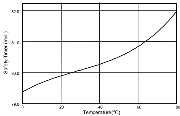
Safety Timer vs Temperature
