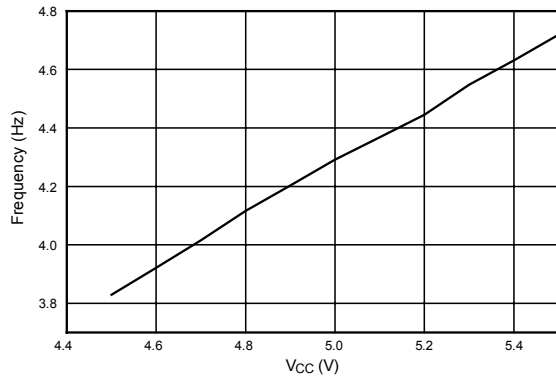
LED Flashing Frequency vs Supply Voltage
