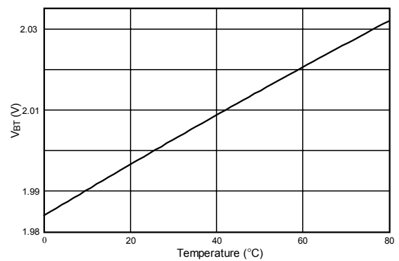
V BT (high) Limit vs Temperature (SEL3<2V)
