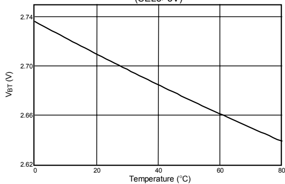
V BT (high) Limit vs Temperature (SEL3>3V)
