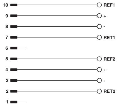
Circuit diagram
