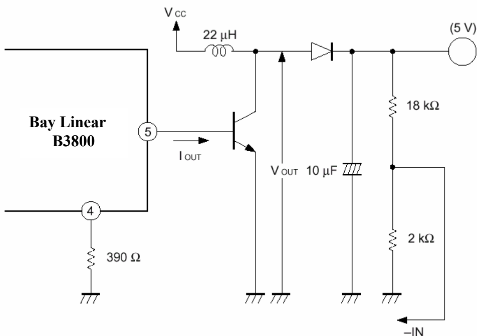
Measurement circuit diagram
