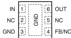
DRV PACKAGE SON-6 (TOP VIEW)
