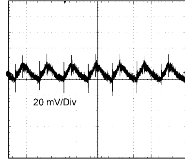
输出波纹 12 V IN , 3.3 V OUT @满负载, BW = 250 MHz
