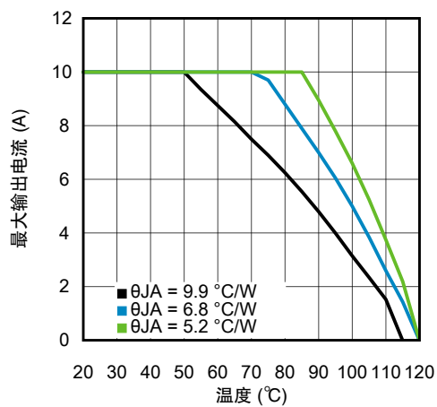
热降额 V_{IN} = 24V , V_{OUT} = 3.3V
