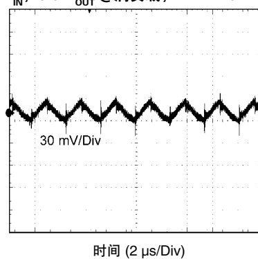
输出波纹 12V_{IN} , 5.0V_{OUT} @满负载, BW = 20 MHz
