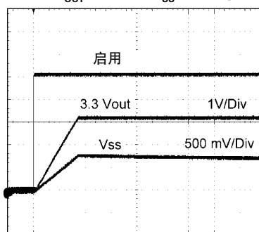
3.3 V OUT 软启动, C SS = 0.47 μF
