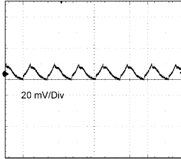
输出波纹 12 V IN , 3.3 V OUT @满负载, BW = 20 MHz
