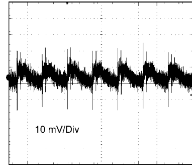
输出波纹 12 V IN , 1.2 V OUT @满负载, BW = 250 MHz
