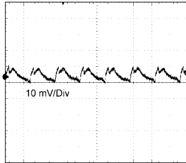
输出波纹 12 V IN , 1.2 V OUT @满负载, BW = 20 MHz
