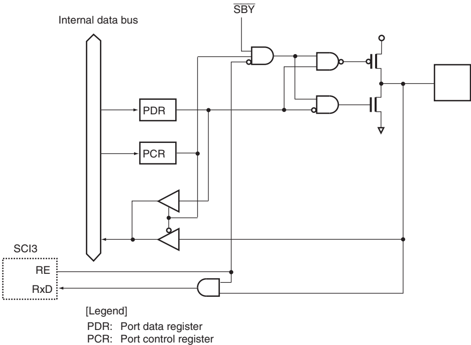
Figure B.6 Port 2 Block Diagram (P21)
