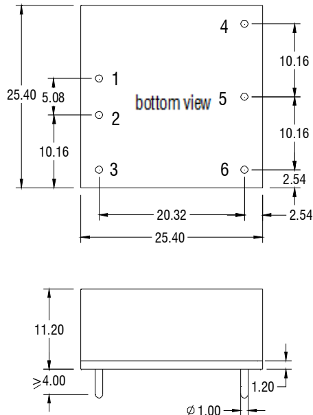
DIP Package
