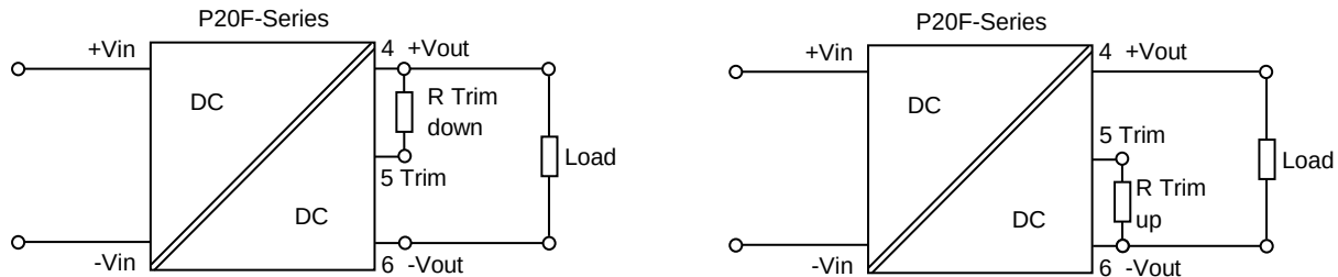
Fig. 4 Output voltage trim application
