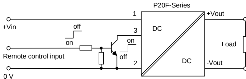
Fig. 5 ON/OFF control application for positive logic
