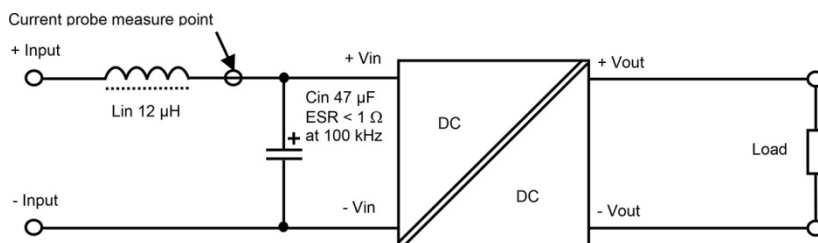
Fig. 2 Measure circuit input ripple current
