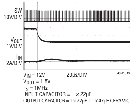
Short-Circuit with No Load Current Applied
