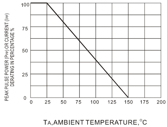
Fig.2 DERATING CURVE
