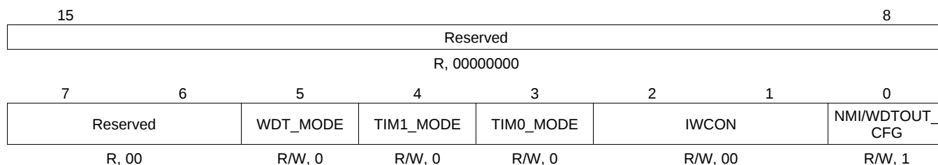
Figure 3-8. Timer Signal Selection Register Layout (0x8000)
