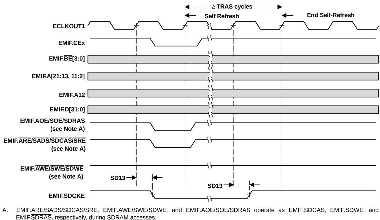
Figure 5-20. SDRAM Self-Refresh Timings
