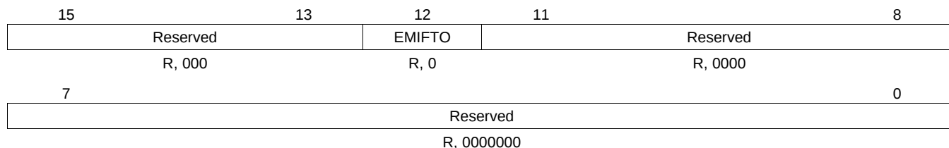
Figure 3-47. DPORT Bus Error Register Layout (0x0202)
