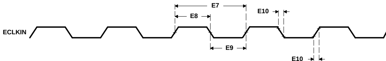
Figure 5-5. ECLKIN Timings for EMIF
