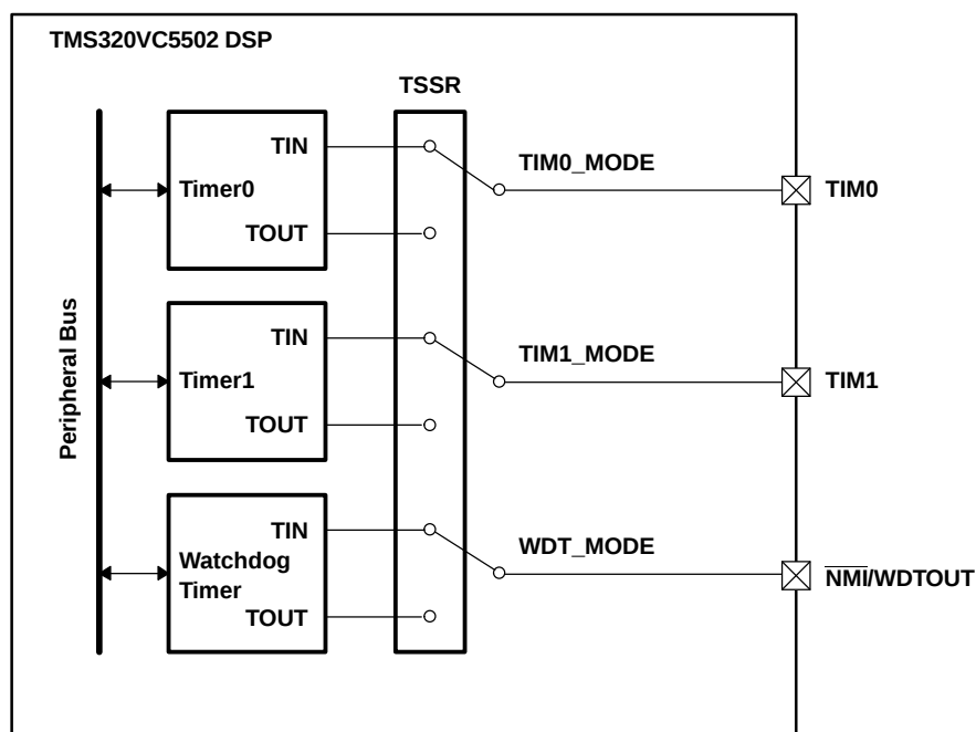
Figure 3-7. Timer Pins
