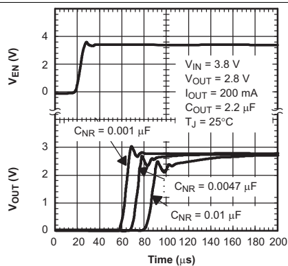
Figure 25. TPS79328 Output Voltage, Enable Voltage vs Time (Start-Up)
