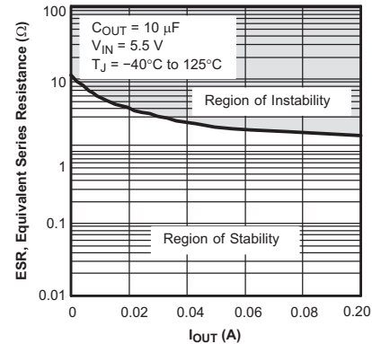
Figure 28. Typical Regions of Stability Equivalent Series Resistance (ESR) vs Output Current
