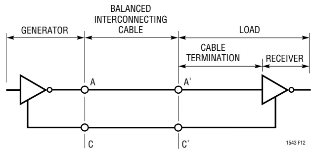
Figure 12. Typical V.10 Interface
