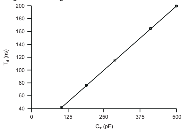
Figure 20. Minimum Dead Time vs C_T
