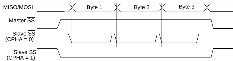
Figure 13. CPHA/SS Timing
