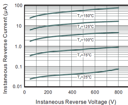
Fig.2 Typical Instaneous Reverse Characteristics
