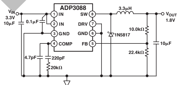
Figure 1. Typical Application
