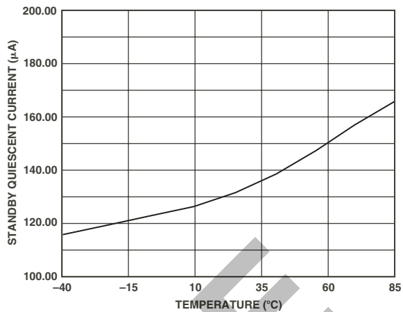
TPC 4. Standby Quiescent Current vs. Temperature
