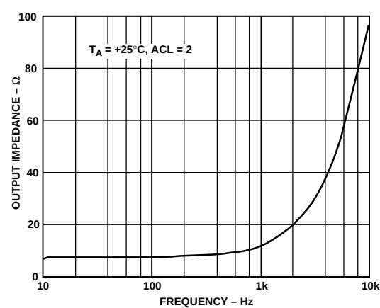
Figure 14. Buffer Amplifier Output Impedance vs. Frequency
