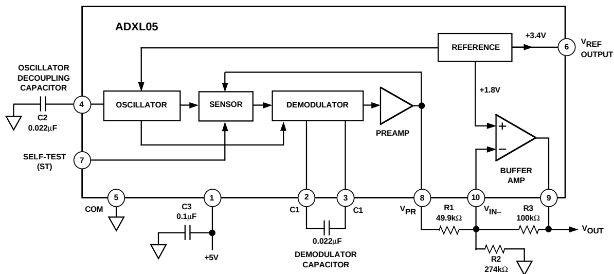
Figure 19. ADXL05 Application Providing an Output Sensitivity of 400\text{ mV/g} , a +2.5\text{ V } 0\text{ g} Level and a Bandwidth of 1\text{ kHz}
