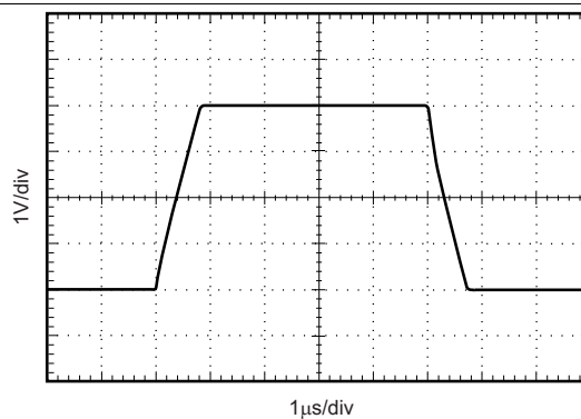
Figure 20. Large-Signal Step Response ( C_L = 100\text{ pF} )
