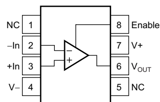
OPA363: D Package 8-Pin SOIC Top View
