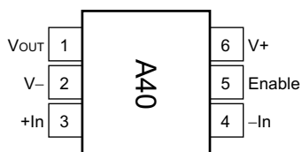
OPA363 (1) : DBV Package 6-Pin SOT-23 Top View
