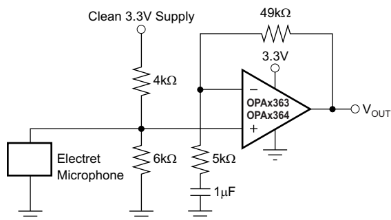
Figure 29. Microphone Preamplifier
