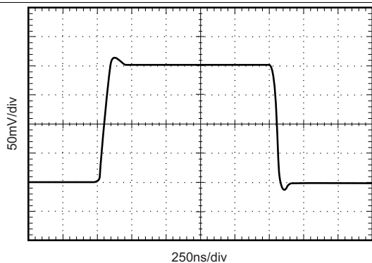
Figure 19. Small-Signal Step Response ( C_L = 100\text{ pF} )
