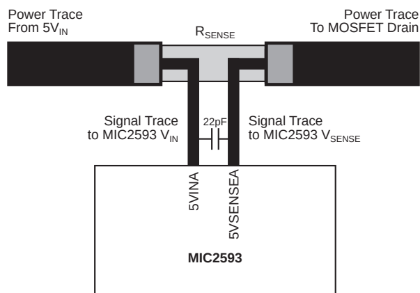
Figure 12. Kelvin Sense Connections for R_{\text{SENSE}} (Applicable to 5V[A/B] and 3V[A/B])
