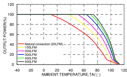
HAE200-48S05W Derating Curve (Note 3) With 0.24" Height Heat-sink
