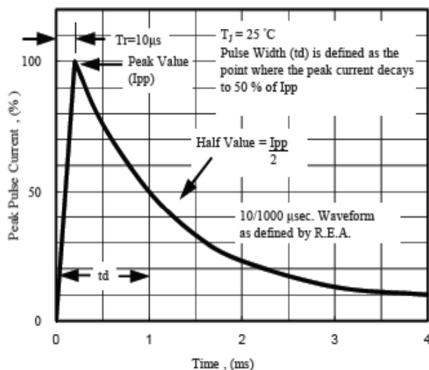
Fig. 5 - Pulse Waveform
