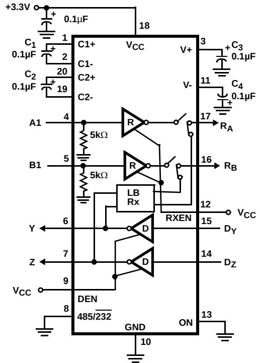
RS-232 MODE WITH LOOPBACK
