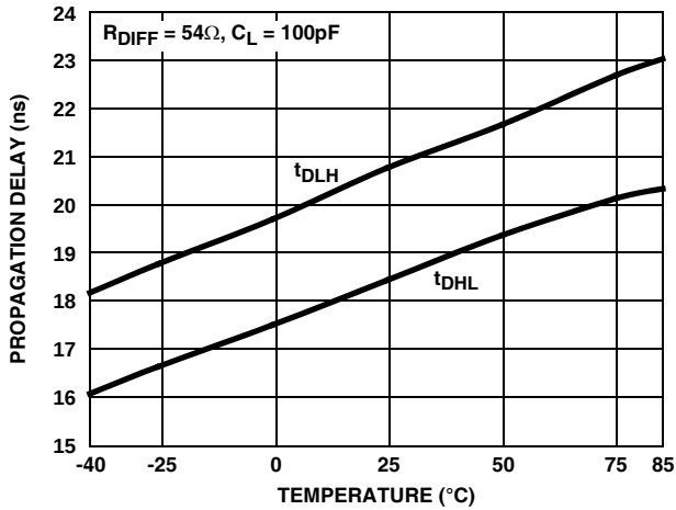
FIGURE 25. RS-485, DRIVER PROPAGATION DELAY vs TEMPERATURE (FAST DATA RATE)
