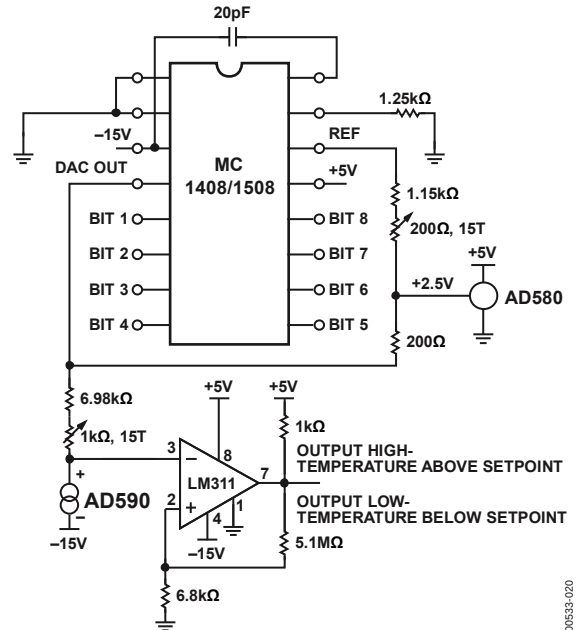
Figure 22. DAC Setpoint
