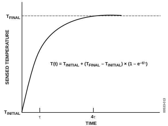
Figure 15. Time Response Curve
