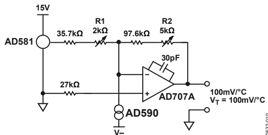
Figure 12. 2-Temperature Trim
