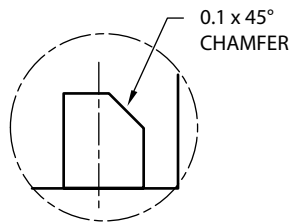
DETAIL A PIN 1 LEAD SCALE 50:1
