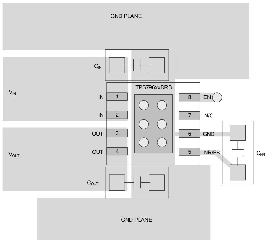
Figure 29. TPS796xx (Fixed Voltage Versions)—DRB Layout Example
