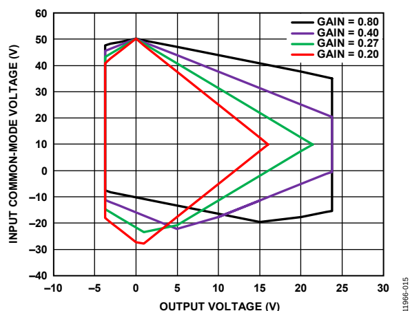
Figure 15. Input Common-Mode Voltage vs. Output Voltage for AVCC = +25\text{ V} and AVEE = -5\text{ V}
