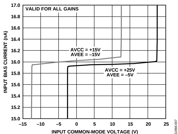
Figure 5. Input Bias Current vs. Input Common-Mode Voltage
