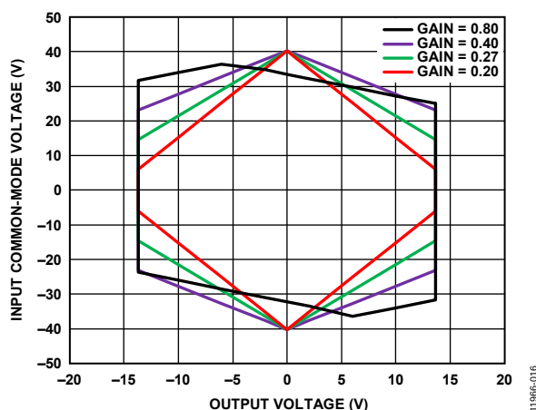
Figure 18. Input Common-Mode Voltage vs. Output Voltage for AVCC = +15\text{ V} and AVEE = -15\text{ V}
