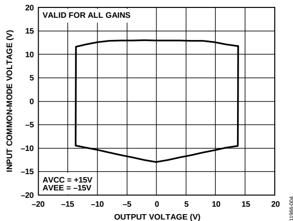
Figure 6. Input Common-Mode Voltage vs. Output Voltage for AV_{CC} = +15\text{ V} and AV_{EE} = -15\text{ V}
