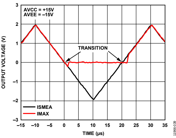
Figure 39. Current Sharing Bus Transition Characteristics
