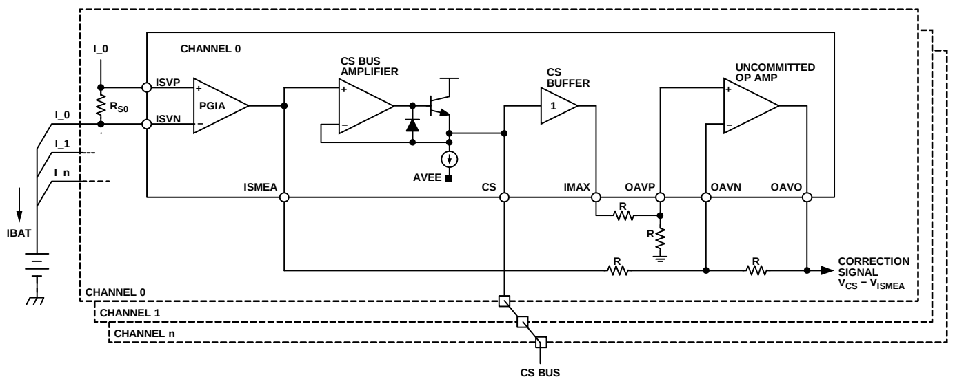
Figure 58. Functional Block Diagram of the Current Sharing Circuit
