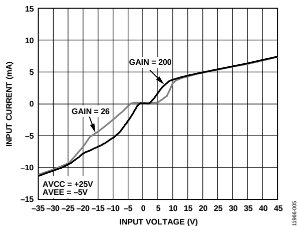
Figure 4. Input Overvoltage Performance for AV_{CC} = +25\text{ V} and AV_{EE} = -5\text{ V}
