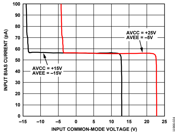
Figure 24. Input Bias Current vs. Input Common-Mode Voltage for Two Supply Voltage Combinations
