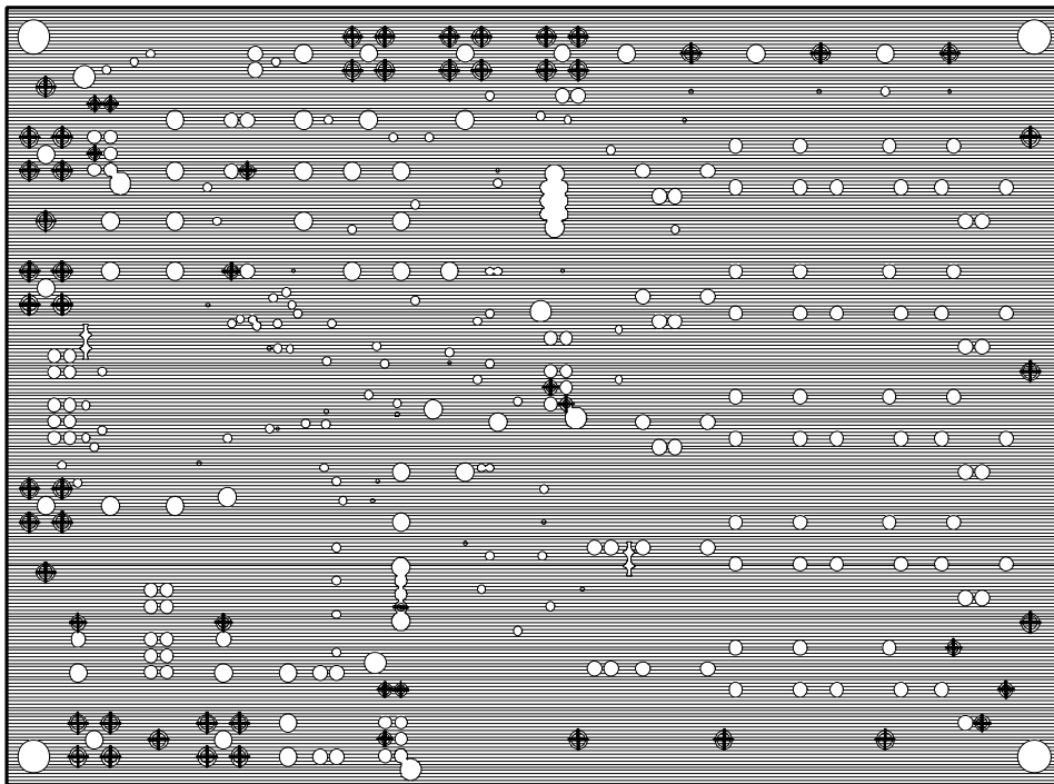
Figure 67. AD8450-EVALZ Ground Plane
