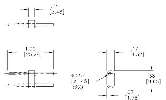
PIN CONNECTOR
