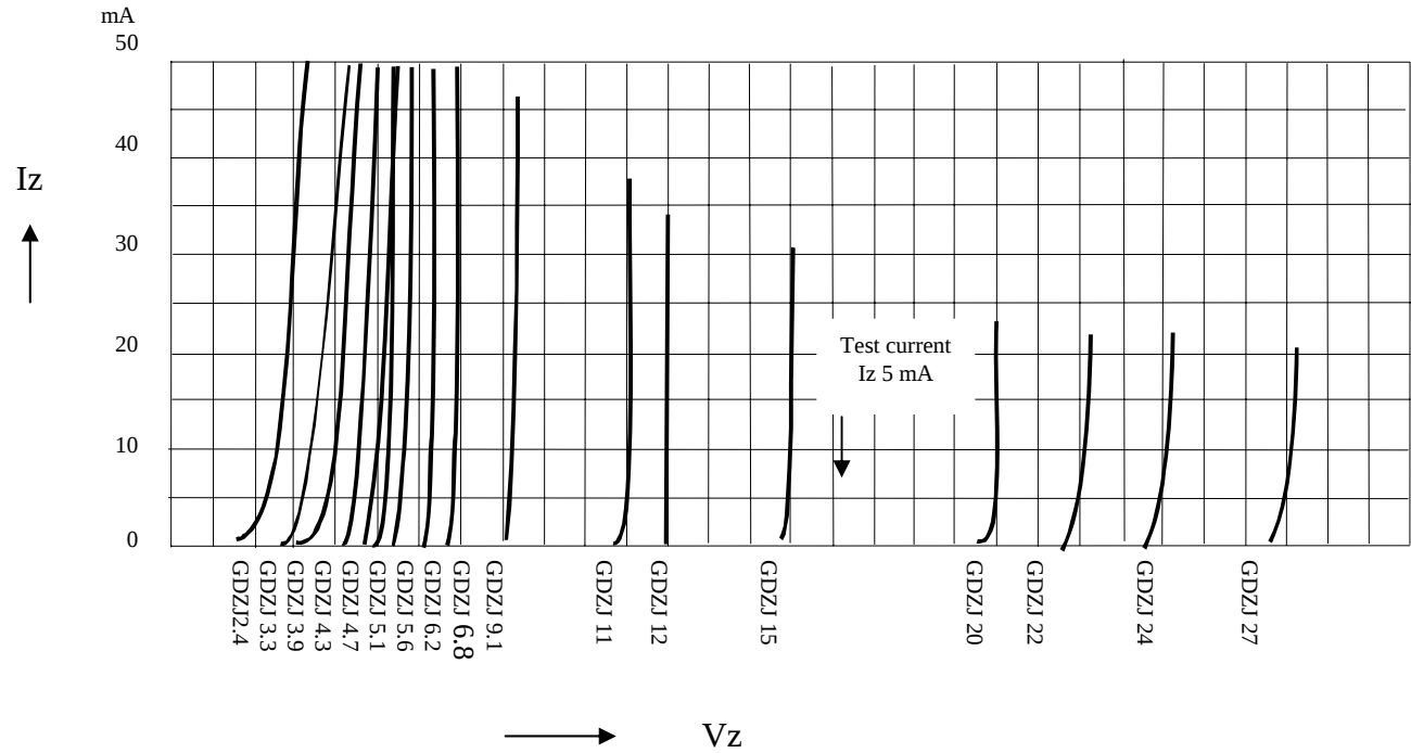
FIG.1- BREAKDOWN CHARACTERISTICS
