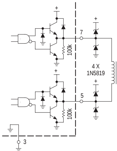
Figure 18. Enhanced System Performance with Common Switching Regulators
