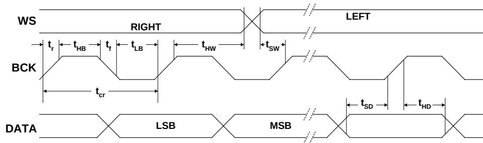
Fig.1 Timing of input signals
