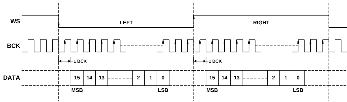
Fig.3 I²S format
