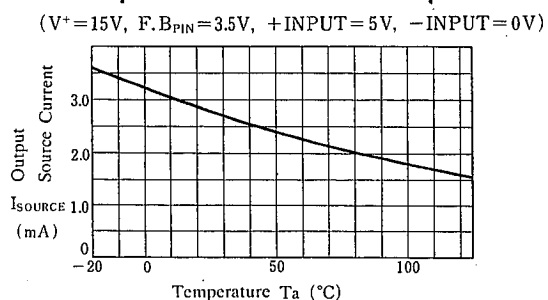
Output Source Current vs. Temperature
