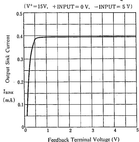
Output Sink Current vs. Feedback Terminal Voltage
