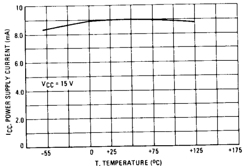
FIGURE 18 – TYPICAL POWER SUPPLY CURRENT versus TEMPERATURE
