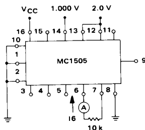
FIGURE 5 – I_6 MEASUREMENT
