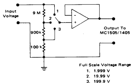
FIGURE 24 – DVM VOLTAGE RANGING
