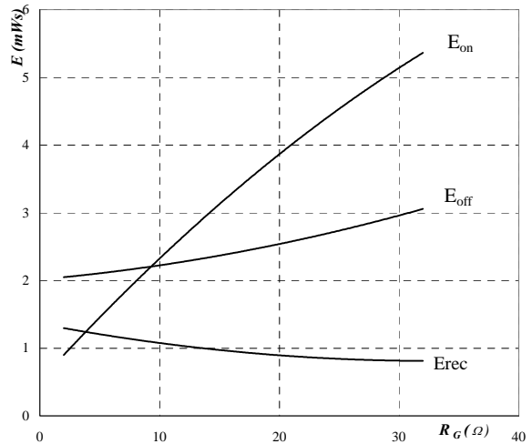
Figure 17. Typical switching energy losses as a function of gate resistor Brake IGBT E = f(R_G)
