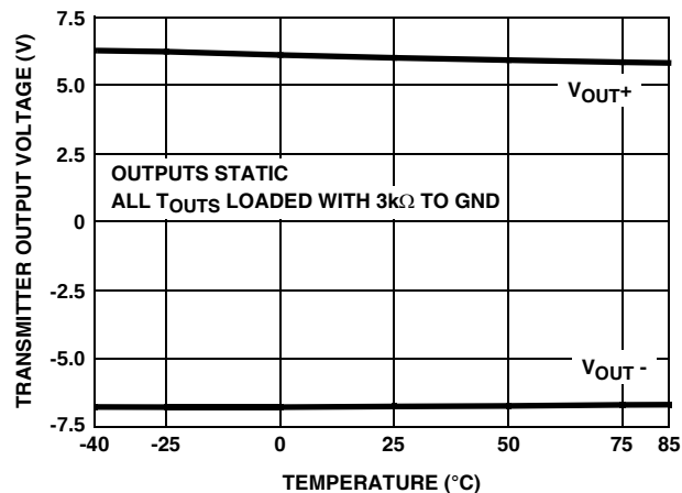
FIGURE 35. RS-232, TRANSMITTER OUTPUT VOLTAGE vs TEMPERATURE
