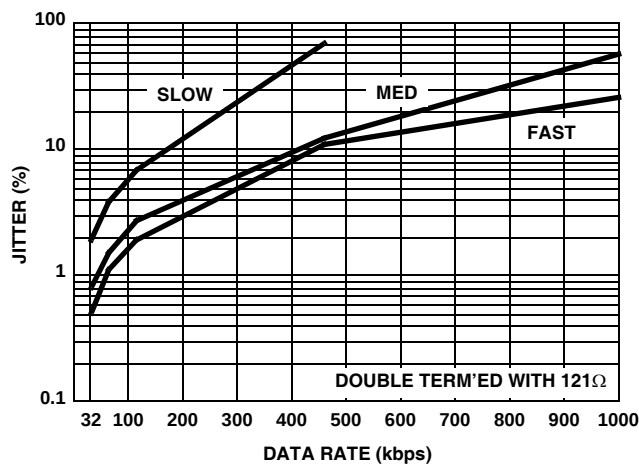
FIGURE 43. RS-485, TRANSMITTER JITTER vs DATA RATE WITH 2000' CAT-5 CABLE
