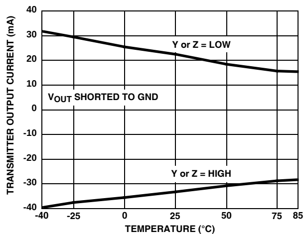
FIGURE 36. RS-232, TRANSMITTER SHORT CIRCUIT CURRENT vs TEMPERATURE
