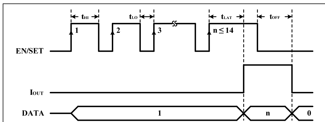
Figure 10 PCC wire Serial Interface Timing
