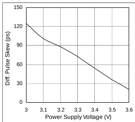
Figure 14. Differential Skew vs. V_{CC} ; Freq = 1MHz
