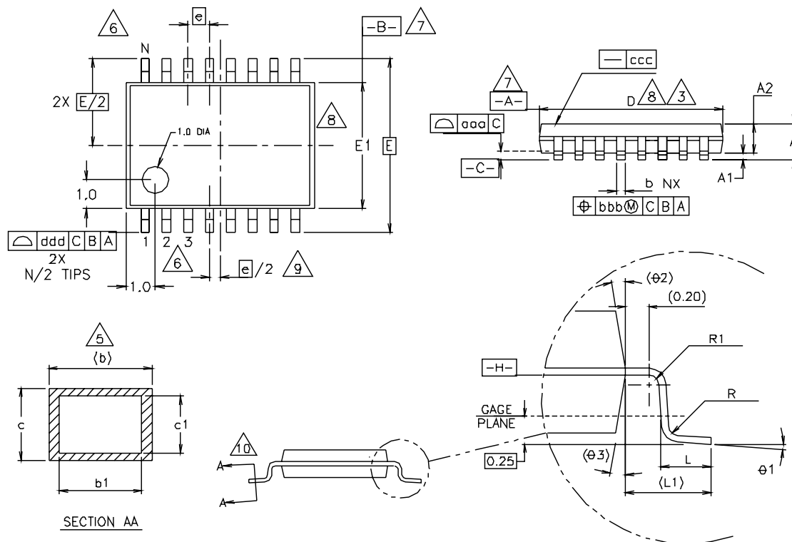
Figure 23. 16-pin TSSOP Package
