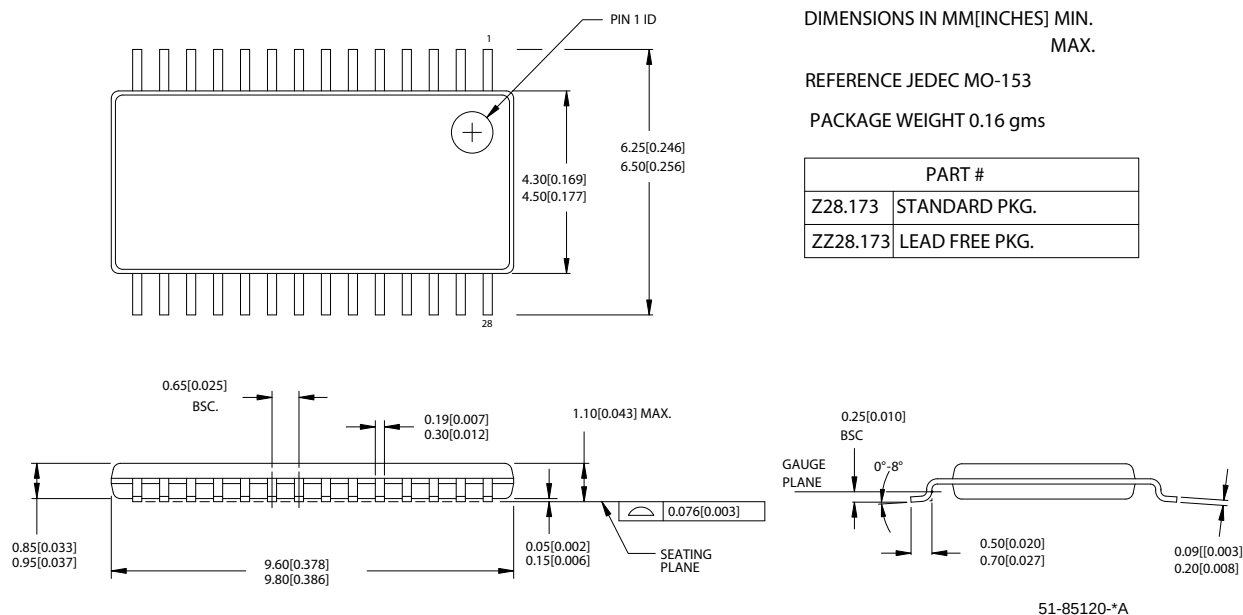
Figure 7. 28-Lead Thin Shrunk Small Outline Package (4.40-mm Body) Z28.173
