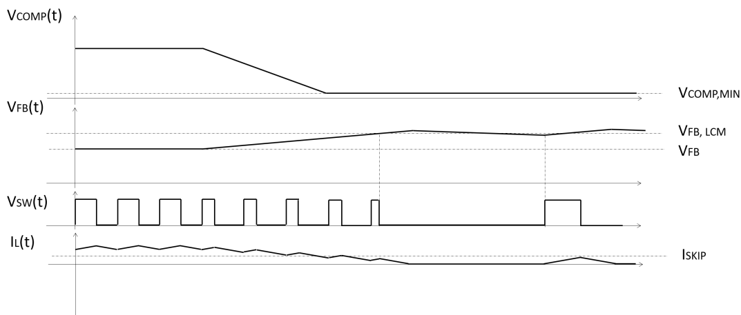
Figure 7. Light-load operation
