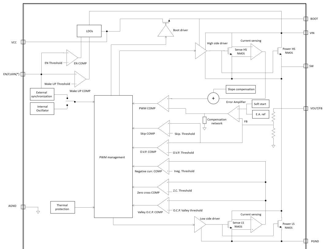
Figure 1. Block diagram
