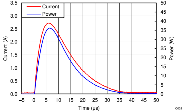
Figure 6-2. Surge Curve (tp = 8/20 μs), Pin IO to GND
