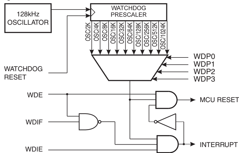
Figure 11-7. Watchdog Timer.
